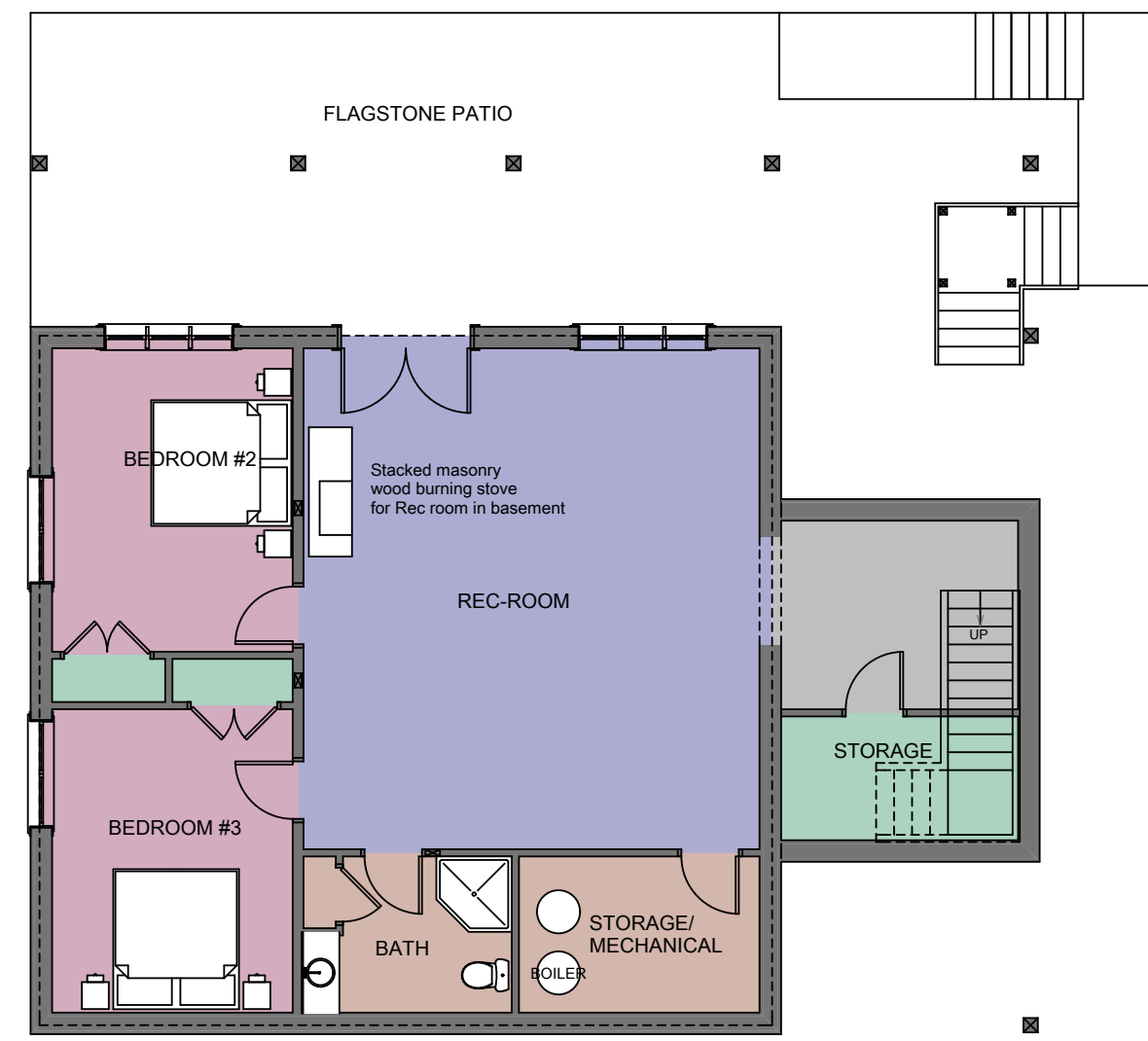
FOUNDATION PLAN W/ BASEMENT LAYOUT AREA: 1302 sq.ft. /121.0 SQ. M
