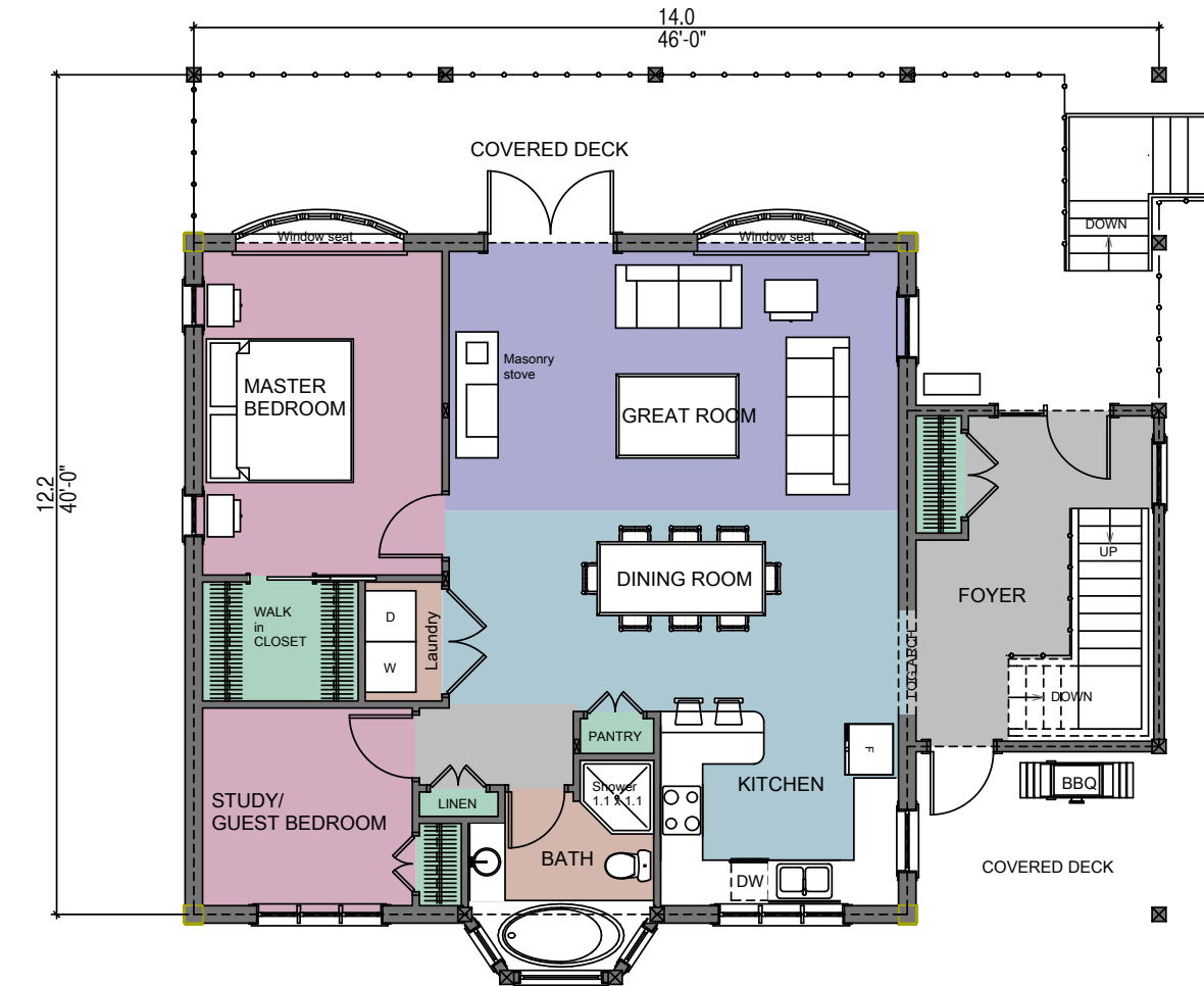
FIRST FLOOR PLAN AREA: 1302 sq.ft./121.0 SQ. M
